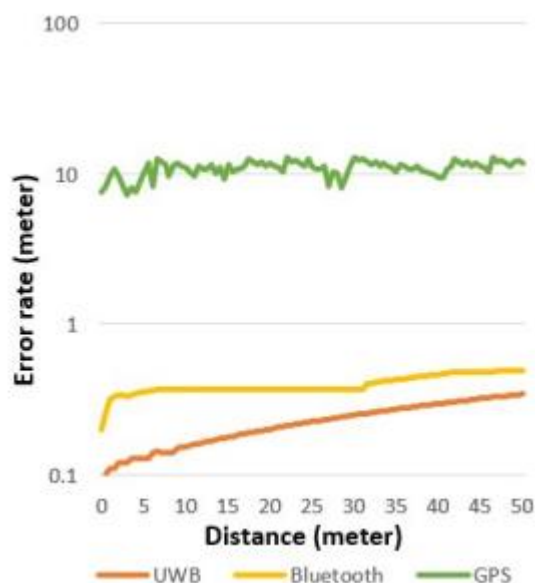
Figure 12: Distance error rate in GPS/Bluetooth/UWB
